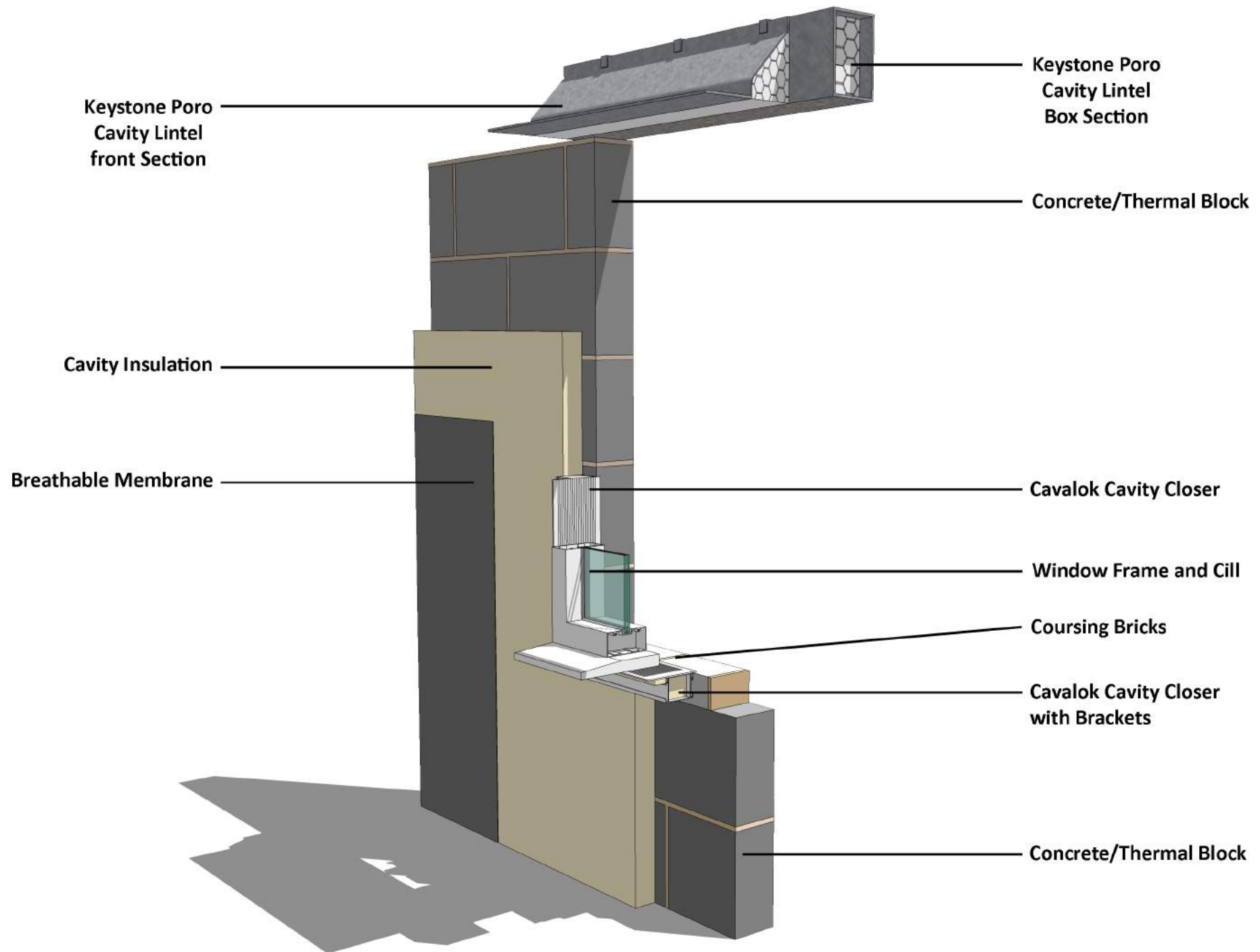
Typical Section through Window without External Brickwork
