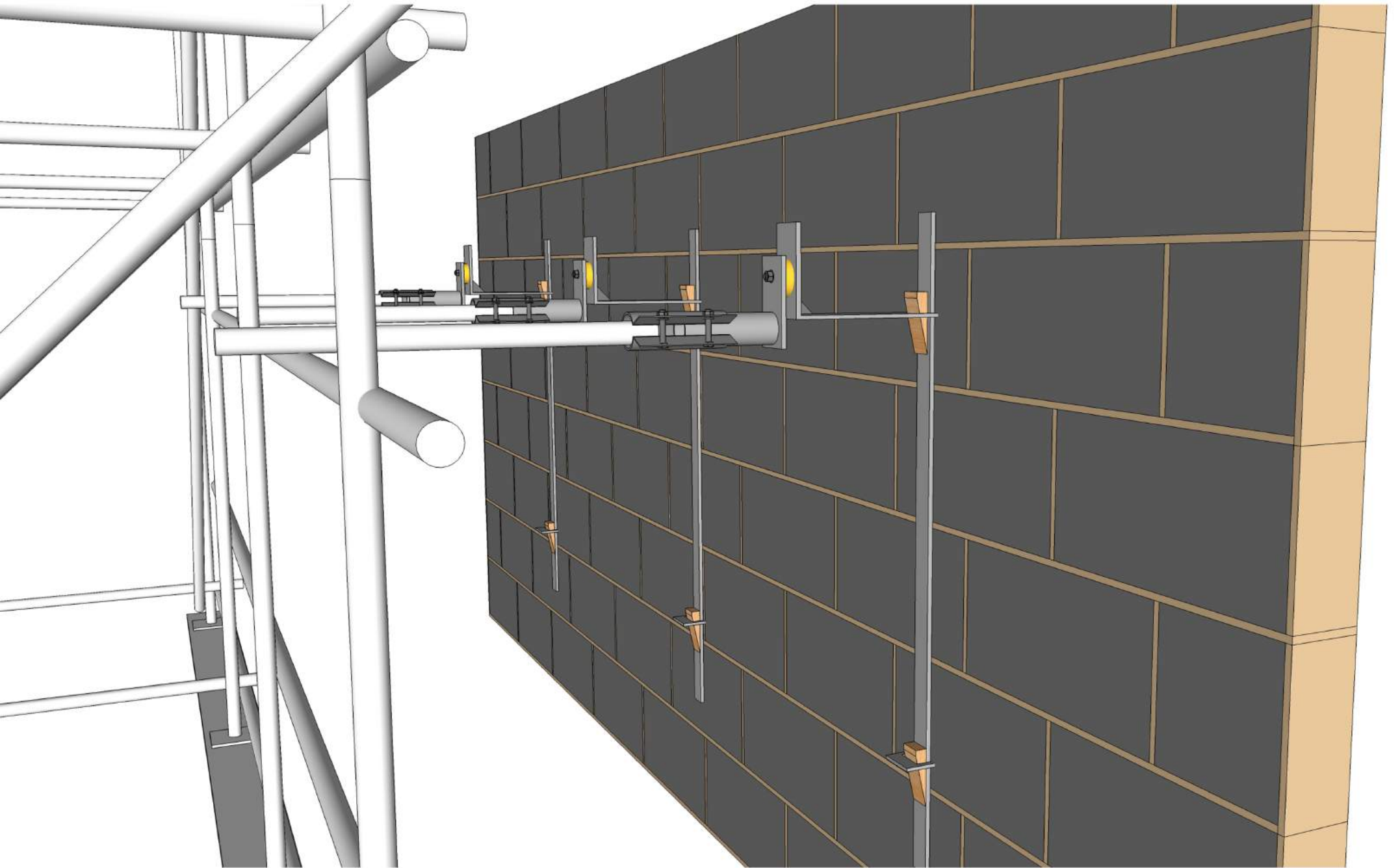
Typical Illustration of RB Components connected to the scaffolding
