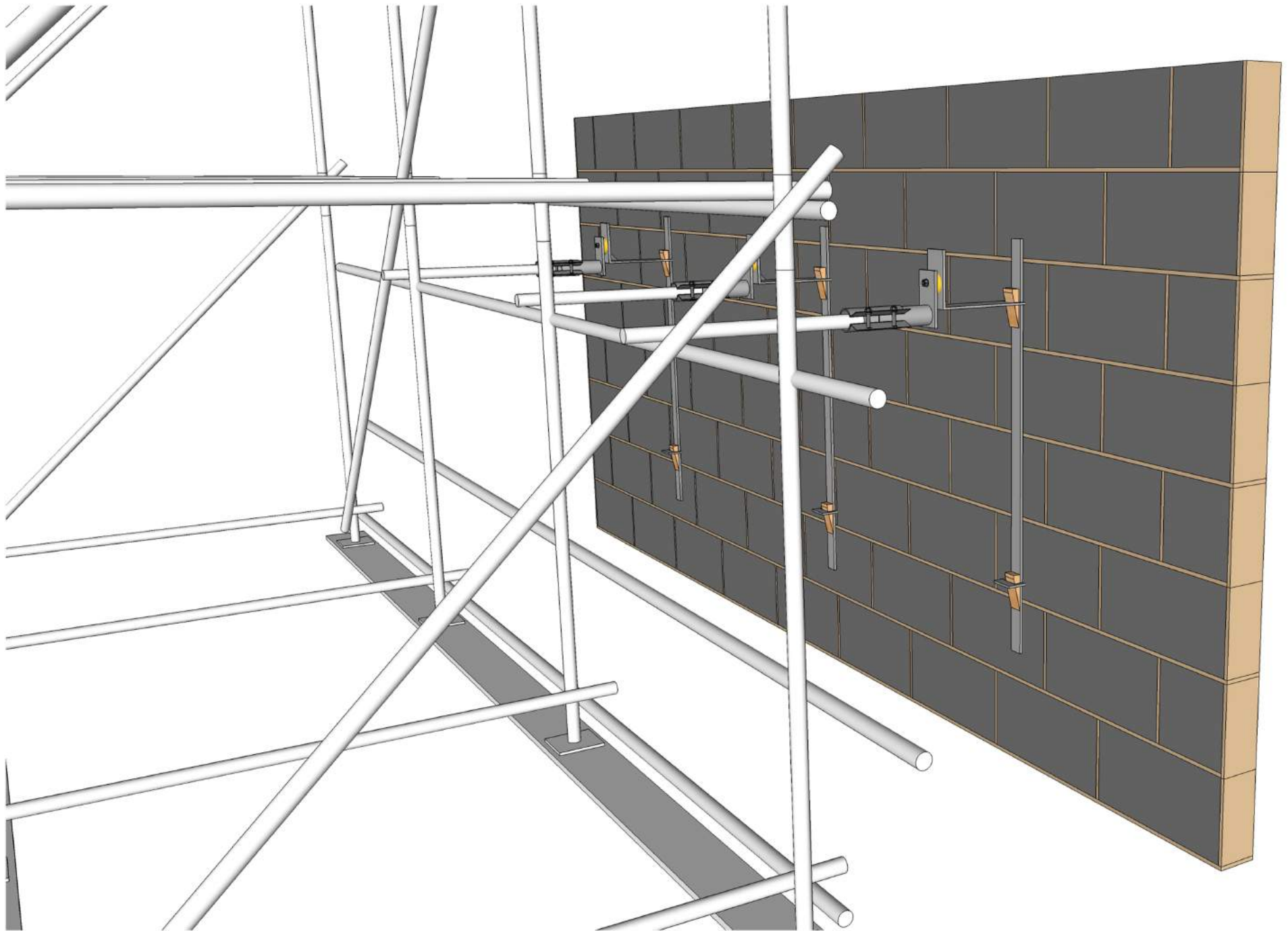
Typical Illustration of RB Components connected to the scaffolding
